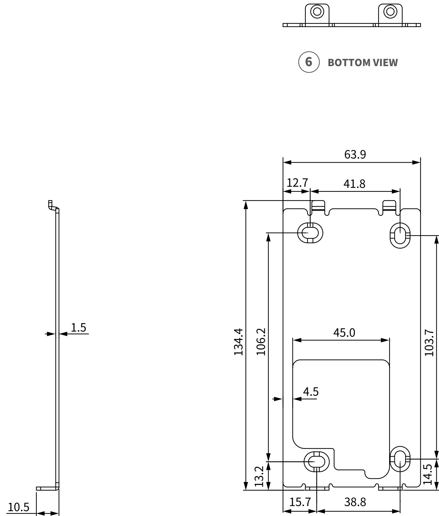
2 RIGHT VIEW
