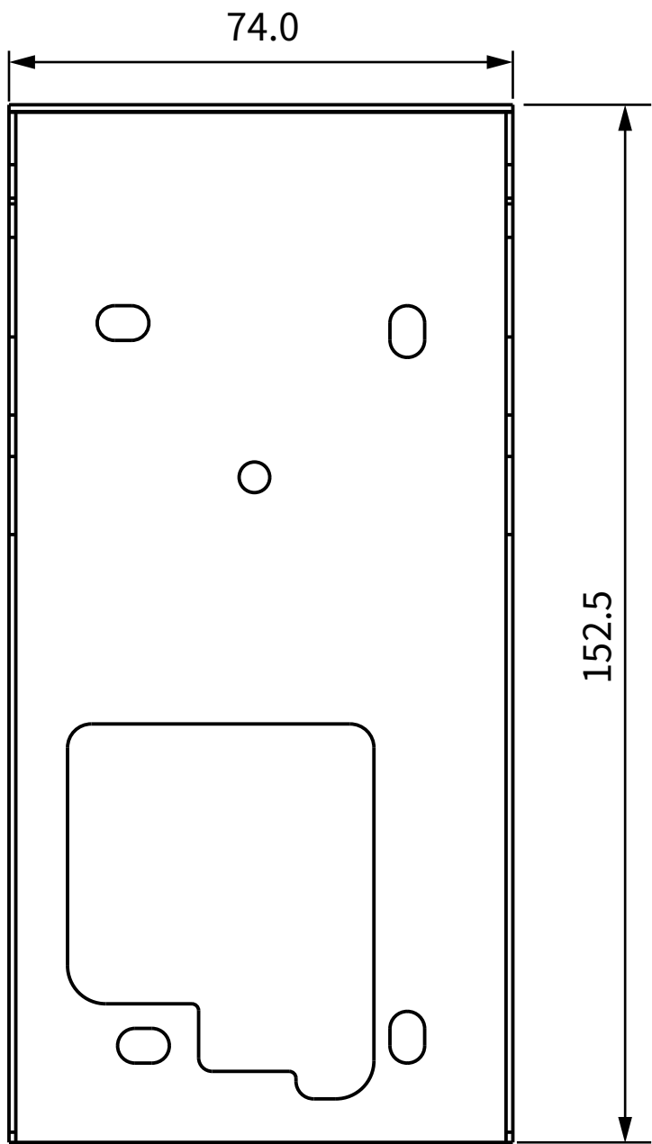
1 FRONT VIEW
