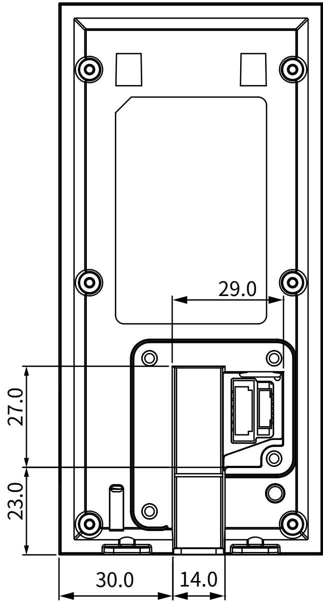
4 BACK VIEW
