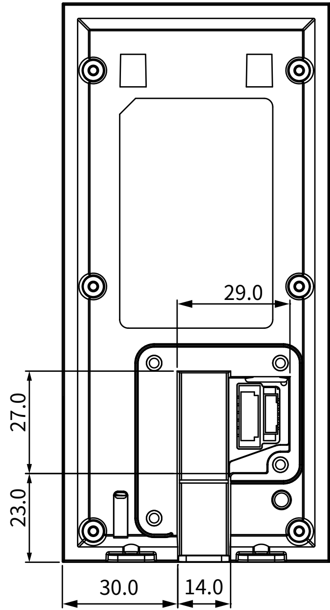
4 BACK VIEW
